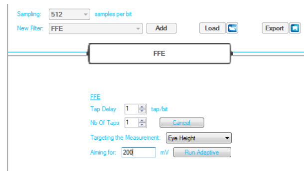
Figure 2: FFE Filter
