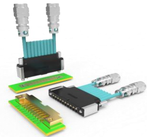
Figure 9: 8 channel coreHC to 1.85mm cable
